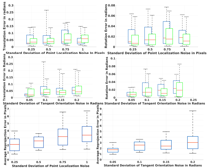
Fig. 6. Pose error between views 1 and 2 (blue) and 1 and 3 (green) vs. feature localization (top) and orientation noise (middle), and point reprojection error vs. localization and orientation noise (bottom).
